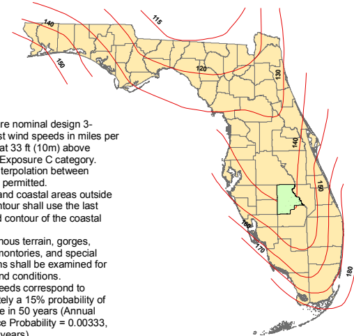
Figure 1609B Ultimate Design Wind Speeds, for Risk Category III and IV Buildings and Other Structures
